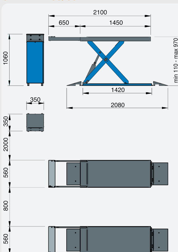
SUPERLIFT 30/35-1X
